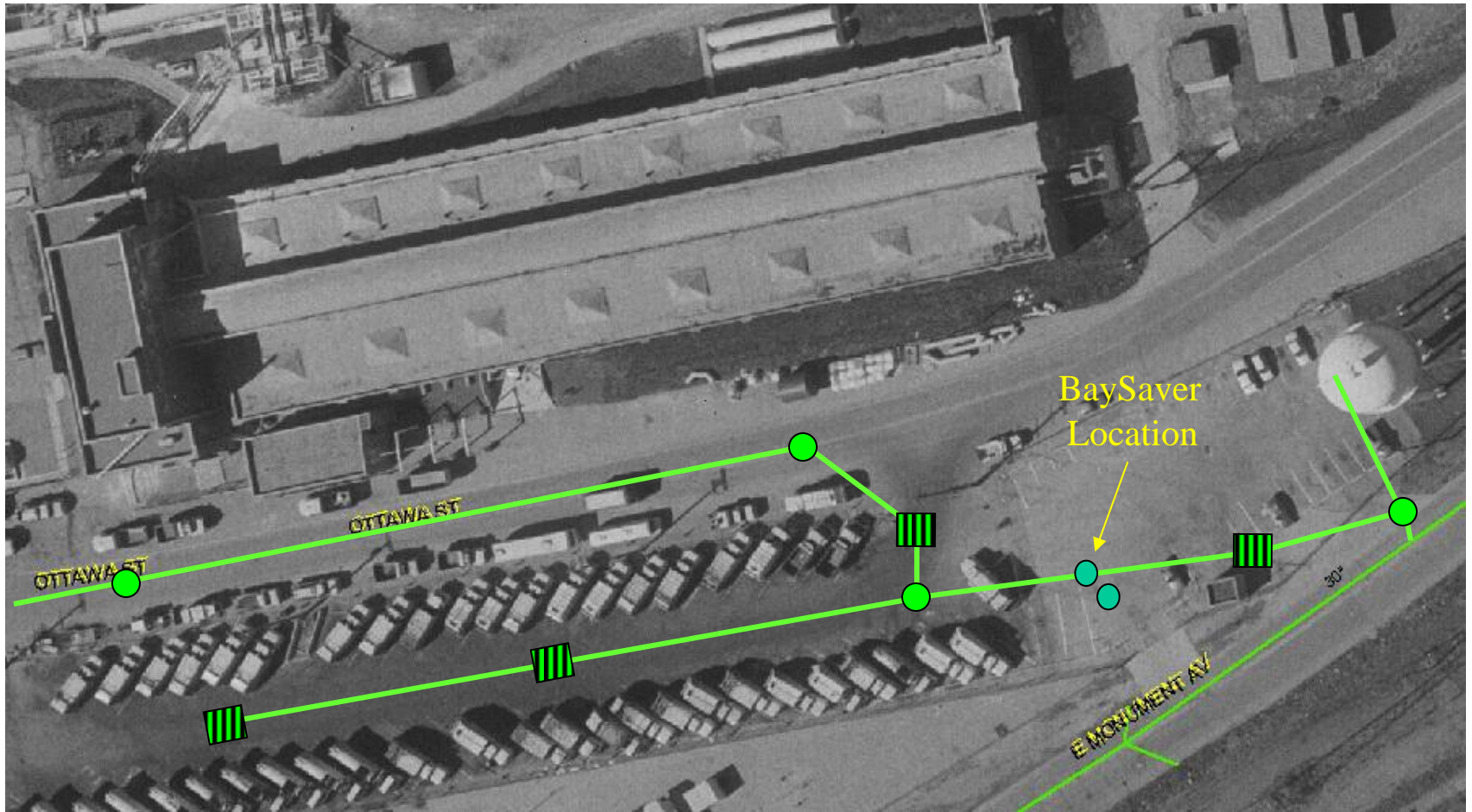
Ottawa Yards Packer Lot BaySaver Separator Project Packer Lot Drainage Area Map Not to Scale
