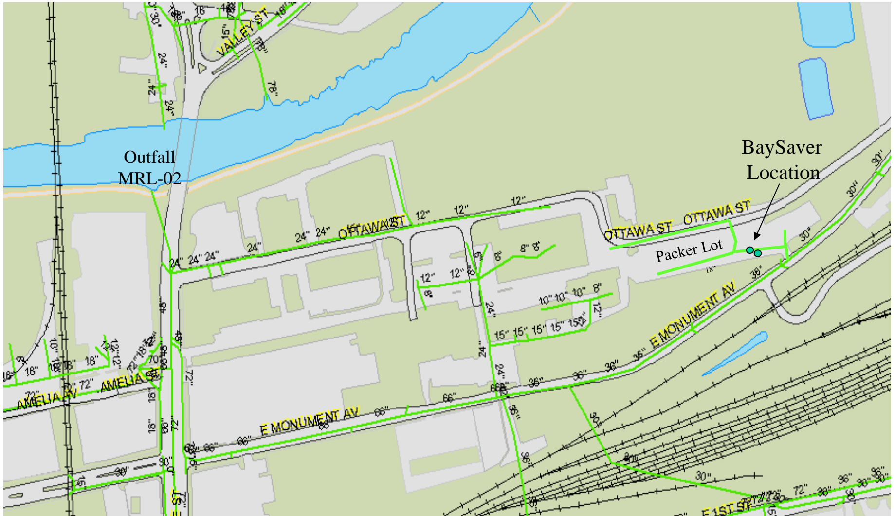
Ottawa Yards Packer Lot BaySaver Separator Project Storm Drainage Area Map Not to Scale
